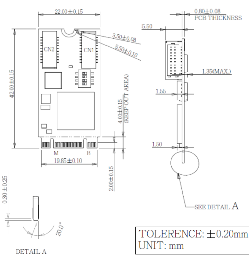
EGP2-X401-W2 (Horizontal Connector)
