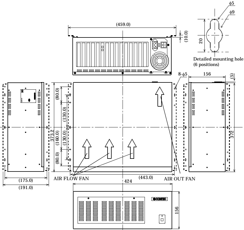
Figure 3.5. Outside Dimensions < ECH(PCI)SF-F13A >
