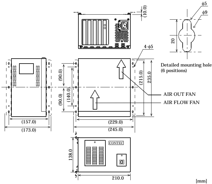
Figure 3.1. Outside Dimensions < ECH(PCI)SF-H4A >
