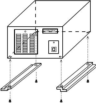
Figure 2.12. Attaching the Rack Mount Brackets
