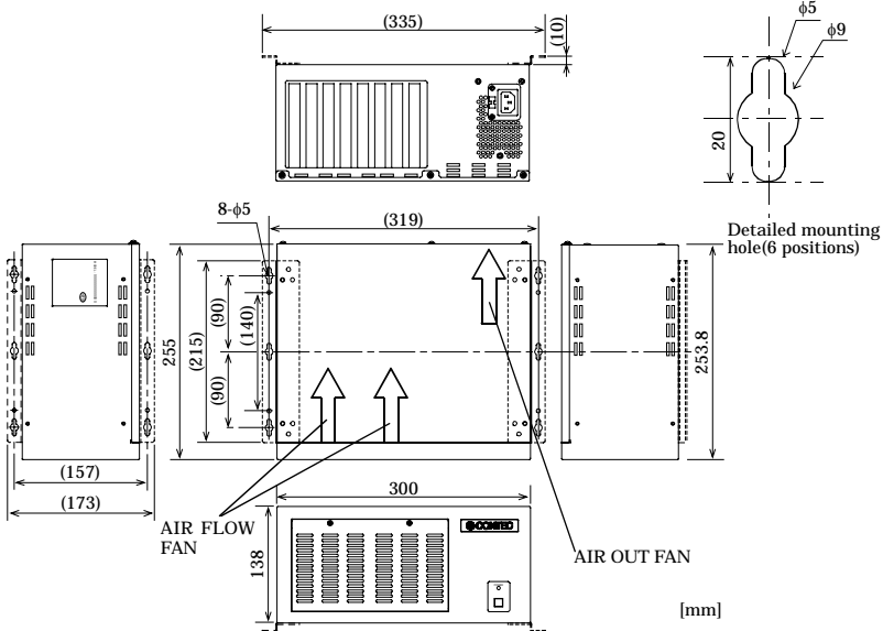
Figure 3.2. Outside Dimensions < ECH(PCI)SF-H7A >
