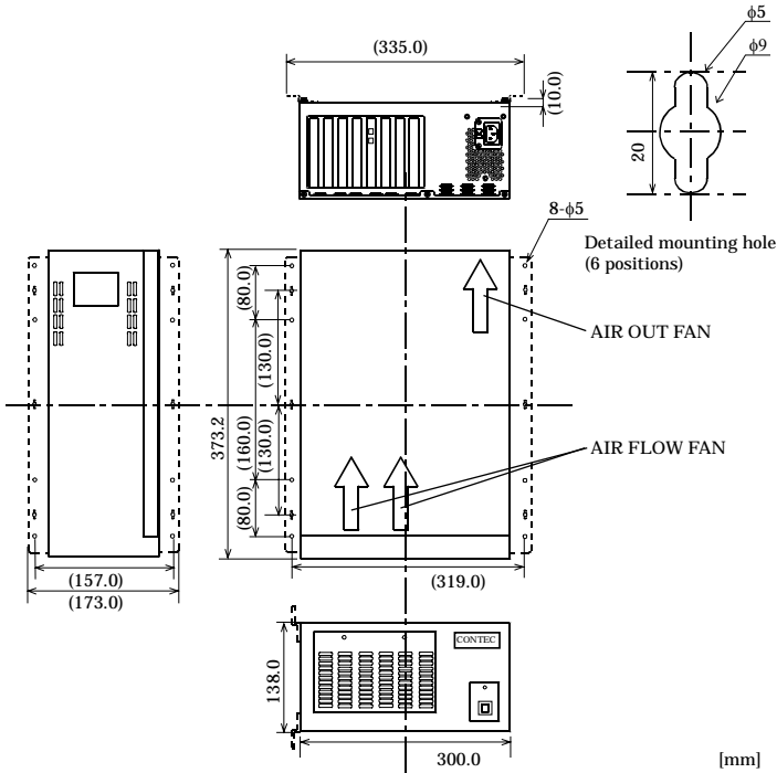
Figure 3.3. Outside Dimensions < ECH(PCI)SF-F7A >
