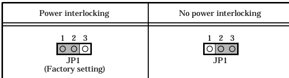
Figure 2.6. Setup for the expansion chassis power interlocking
