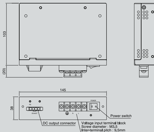
IPC - POA100SH (Power supply)
