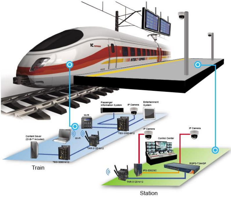
Networking connections
