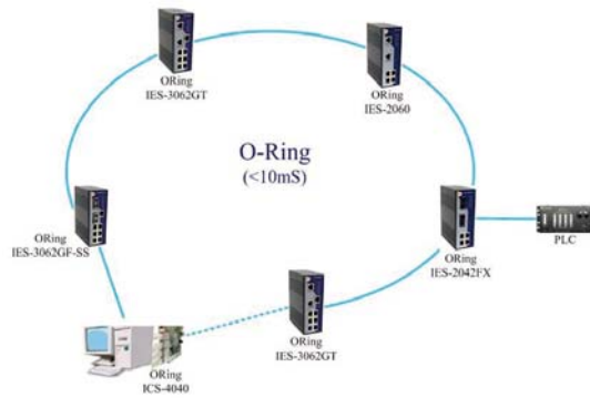
Network connection
